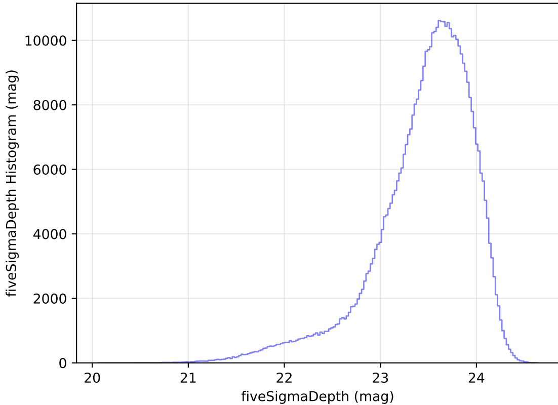
internal_u_expt45_nscale1.2v3.4_10yrs WFD i band: fiveSigmaDepth Histogram
