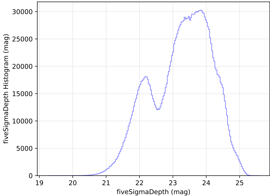
internal_u_expt45_nscale1.2v3.4_10yrs WFD all bands: fiveSigmaDepth Histogram
