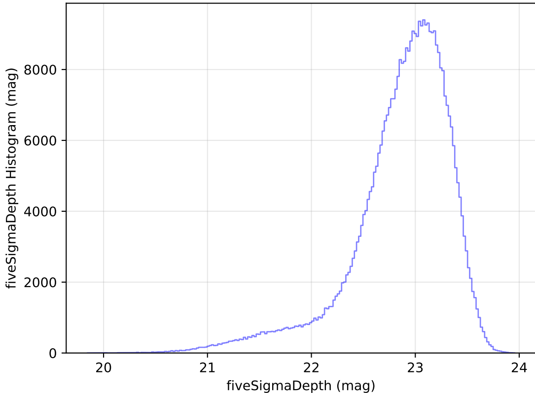
internal_u_expt45_nscale1.2v3.4_10yrs All sky z band: fiveSigmaDepth Histogram
