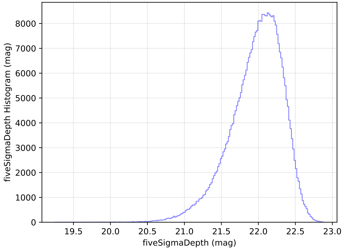
internal_u_expt45_nscale1.2v3.4_10yrs All sky y band: fiveSigmaDepth Histogram
