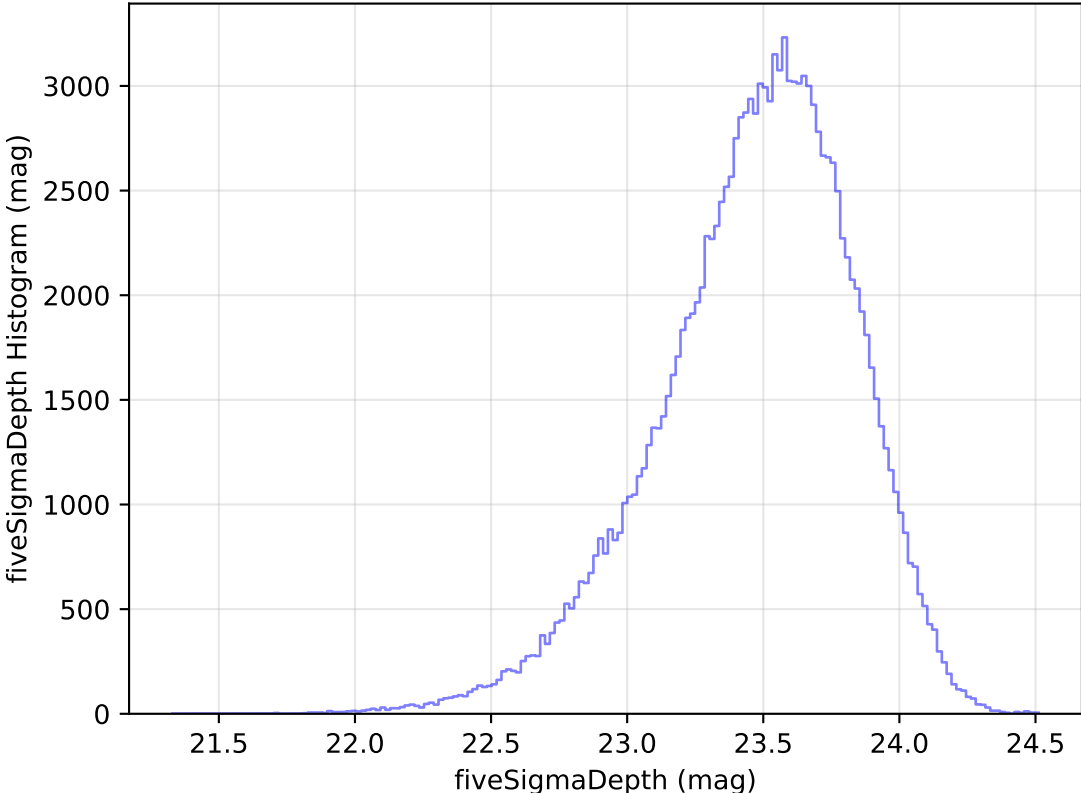
internal_u_expt45_nscale1.2v3.4_10yrs All sky u band: fiveSigmaDepth Histogram
