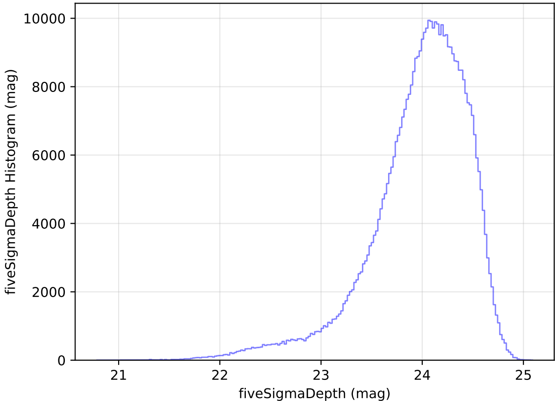
internal_u_expt45_nscale1.2v3.4_10yrs All sky r band: fiveSigmaDepth Histogram
