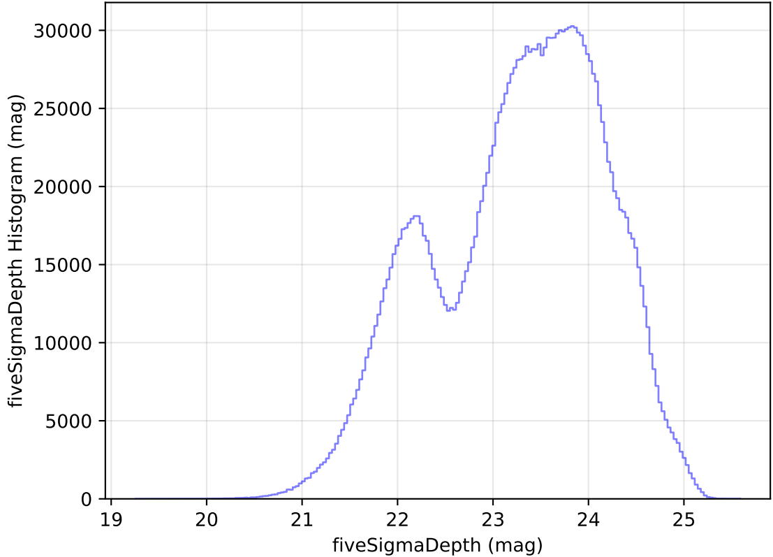
internal_u_expt45_nscale1.2v3.4_10yrs All sky all bands: fiveSigmaDepth Histogram
