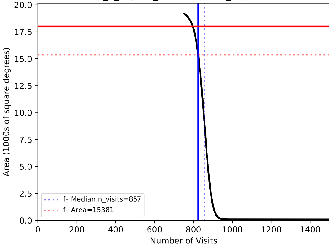
internal_u_expt45_nscale1.2v3.4_10yrs WFD: fO
