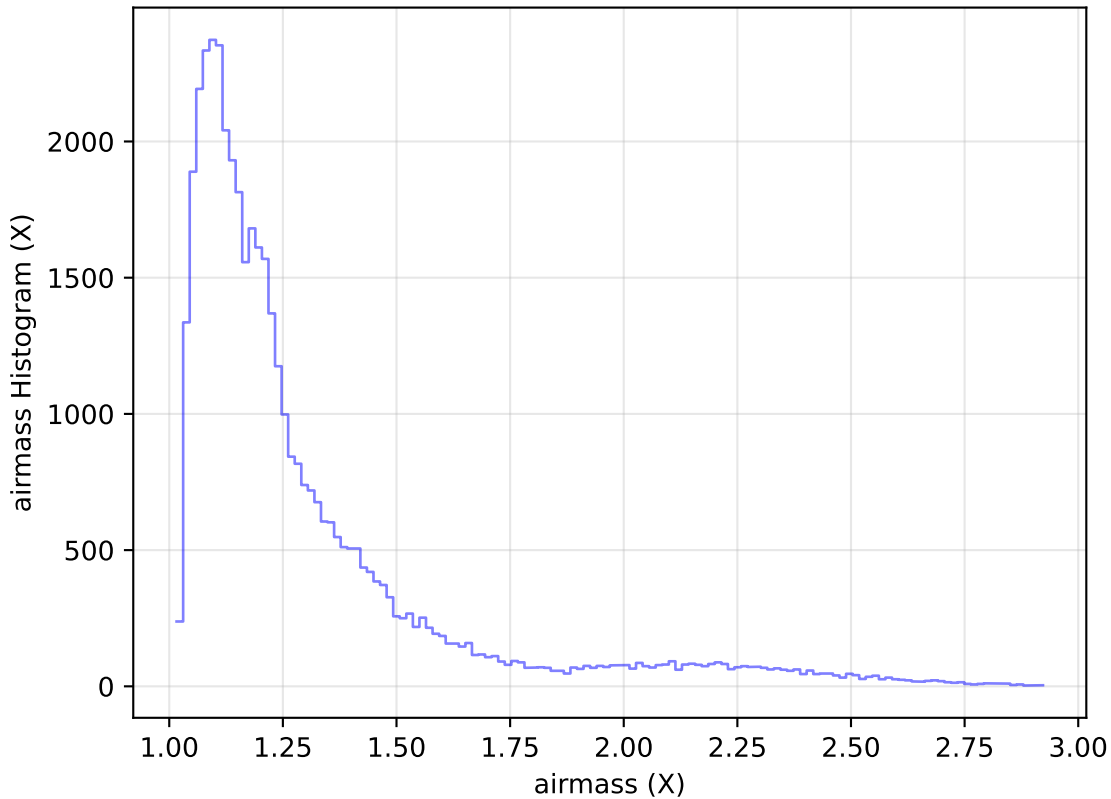
internal_u_expt45_nscale1.2v3.4_10yrs Yr 1 z band: airmass Histogram
