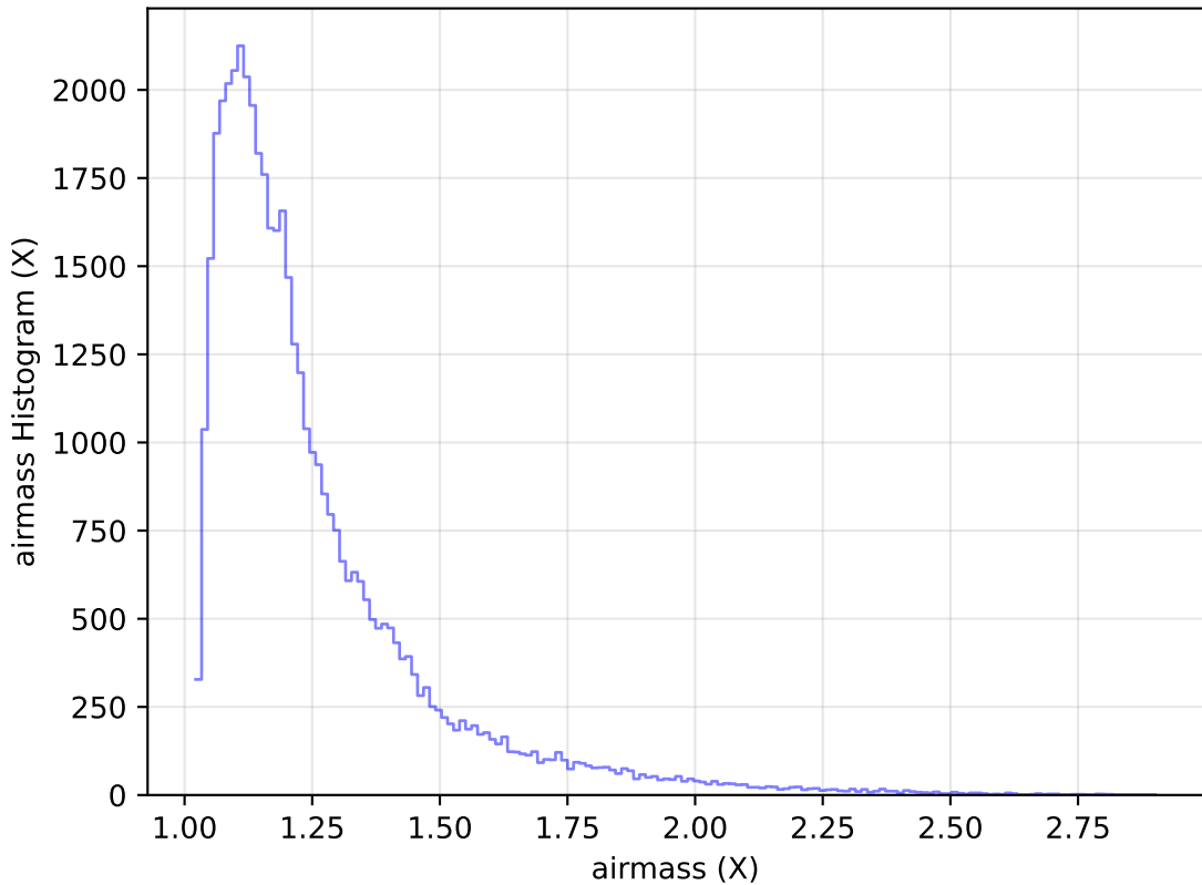
internal_u_expt45_nscale1.2v3.4_10yrs Yr 1 y band: airmass Histogram
