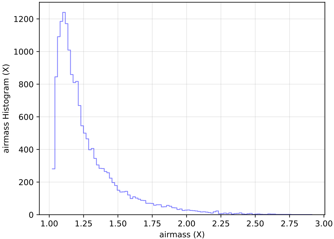
internal_u_expt45_nscale1.2v3.4_10yrs Yr 1 u band: airmass Histogram
