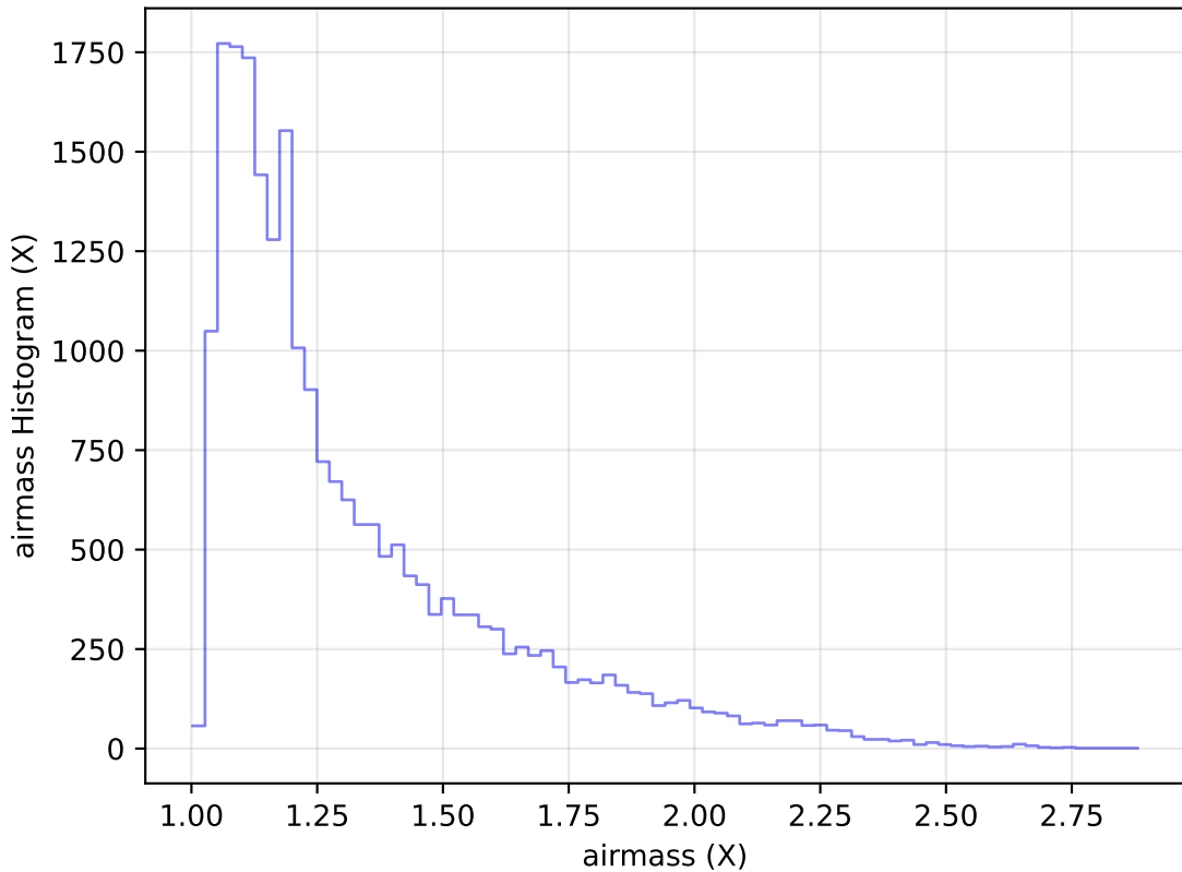
internal_u_expt45_nscale1.2v3.4_10yrs Yr 1 g band: airmass Histogram
