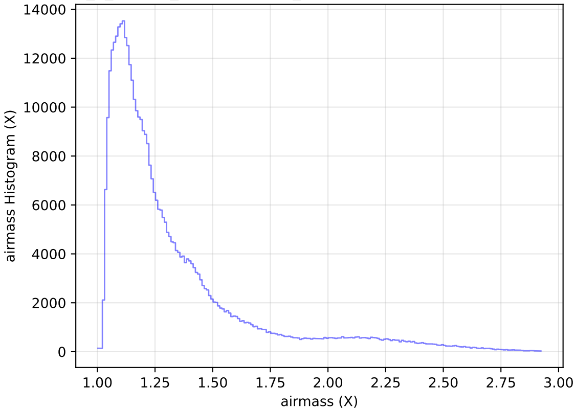
internal_u_expt45_nscale1.2v3.4_10yrs WFD z band: airmass Histogram
