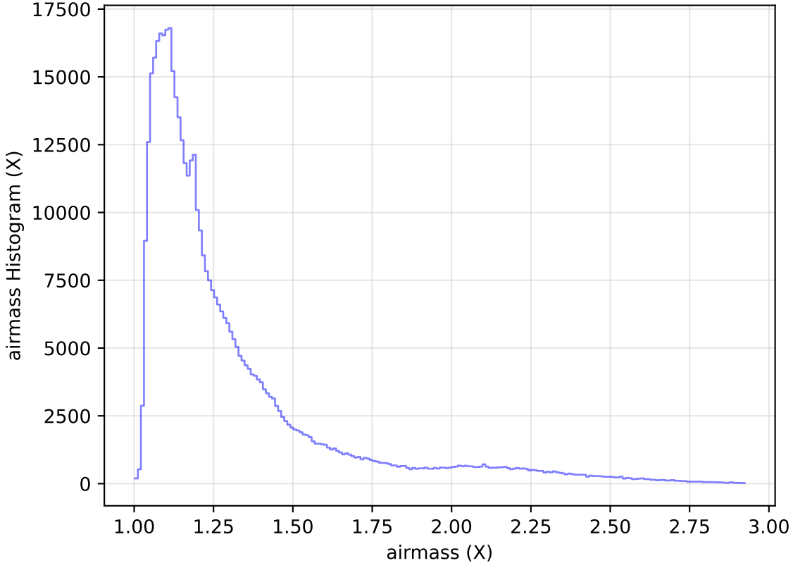
internal_u_expt45_nscale1.2v3.4_10yrs WFD i band: airmass Histogram
