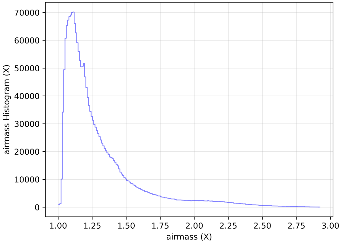
internal_u_expt45_nscale1.2v3.4_10yrs WFD all bands: airmass Histogram
