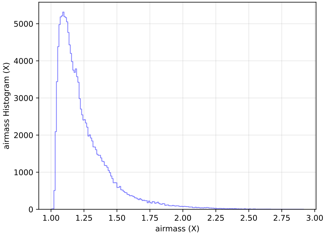
internal_u_expt45_nscale1.2v3.4_10yrs All sky u band: airmass Histogram
