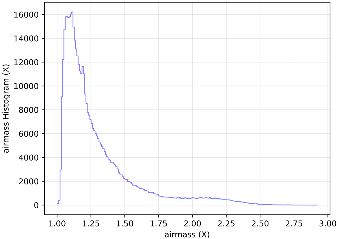
internal_u_expt45_nscale1.2v3.4_10yrs All sky r band: airmass Histogram
