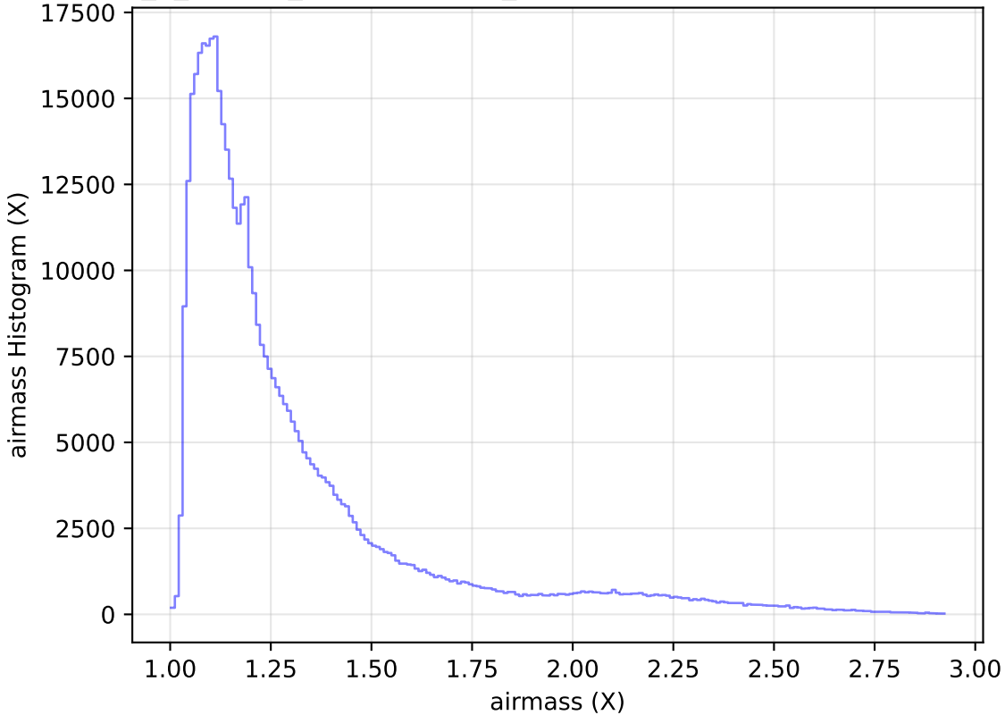
internal_u_expt45_nscale1.2v3.4_10yrs All sky i band: airmass Histogram
