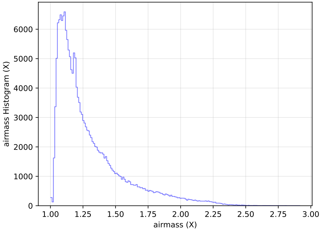
internal_u_expt45_nscale1.2v3.4_10yrs All sky g band: airmass Histogram
