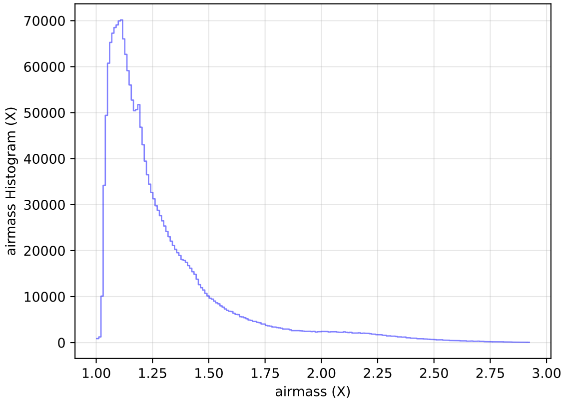
internal_u_expt45_nscale1.2v3.4_10yrs All sky all bands: airmass Histogram
