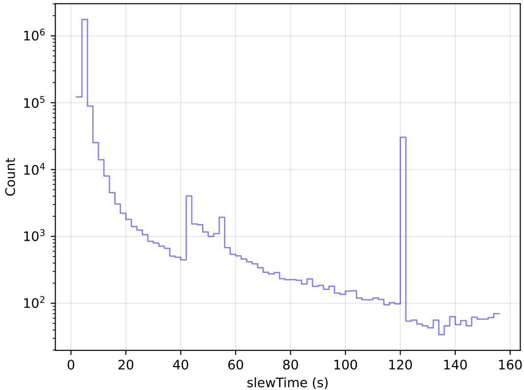
internal_u_expt45_nscale1.2v3.4_10yrs All visits: Slew Time Histogram
