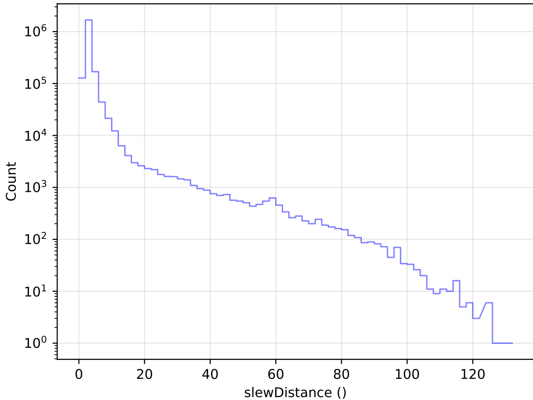
internal_u_expt45_nscale1.2v3.4_10yrs All visits: Slew Distance Histogram
