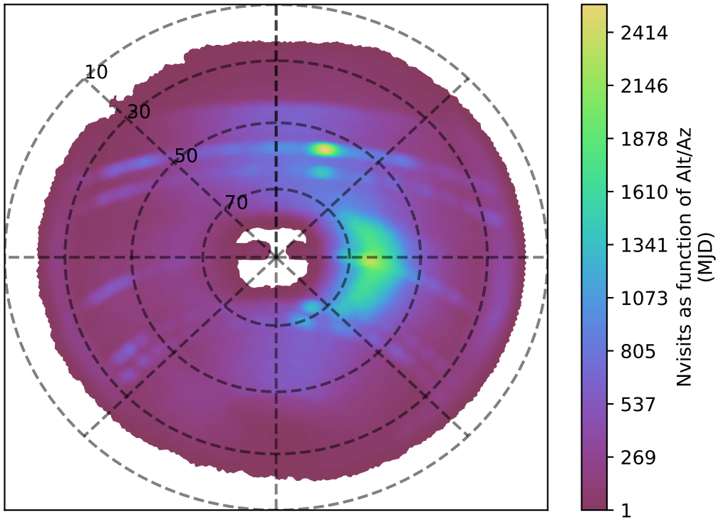
internal_u_expt45_nscale1.2v3.4_10yrs z band: Nvisits as function of Alt/Az
