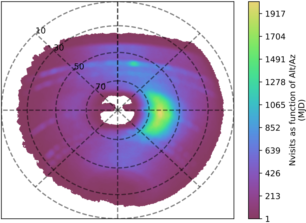
internal_u_expt45_nscale1.2v3.4_10yrs y band: Nvisits as function of Alt/Az
