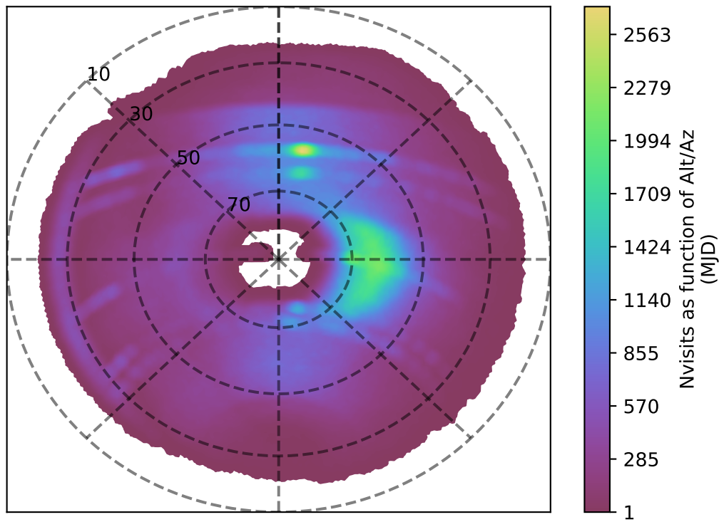
internal_u_expt45_nscale1.2v3.4_10yrs r band: Nvisits as function of Alt/Az
