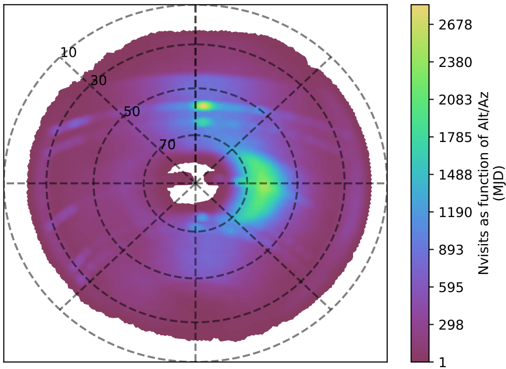
internal_u_expt45_nscale1.2v3.4_10yrs i band: Nvisits as function of Alt/Az
