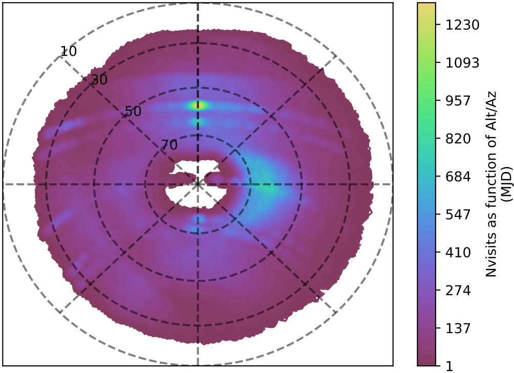
internal_u_expt45_nscale1.2v3.4_10yrs g band: Nvisits as function of Alt/Az
