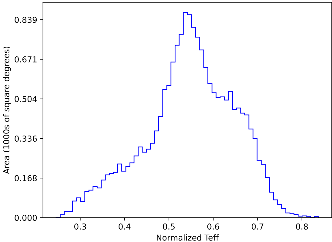
internal_u_expt45_nscale1.2v3.4_10yrs WFD y band: Normalized Teff
