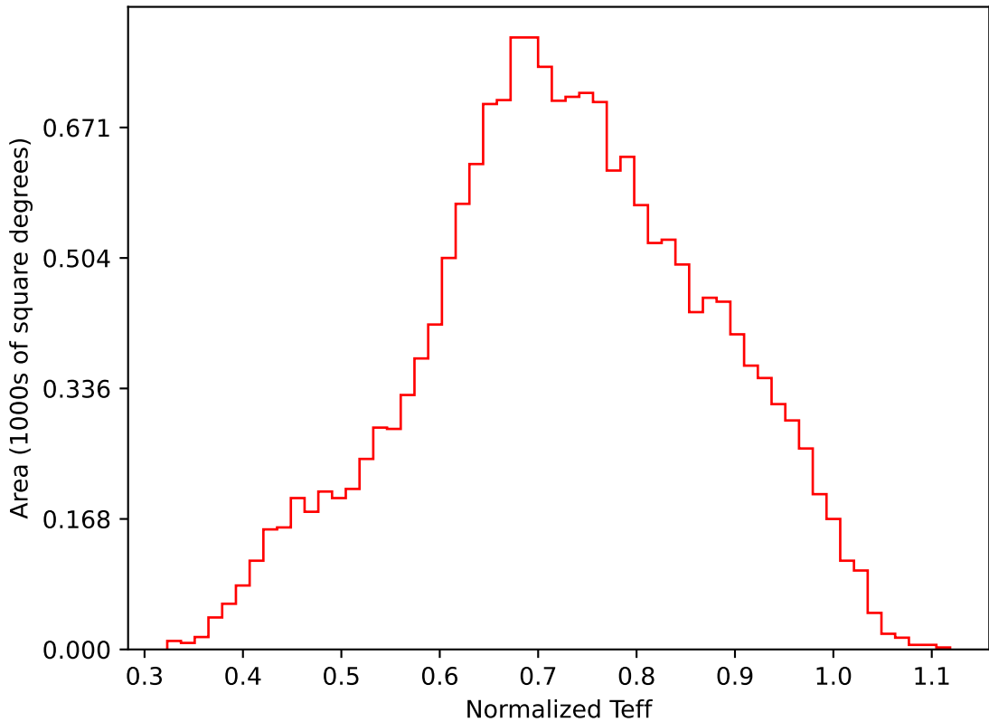
internal_u_expt45_nscale1.2v3.4_10yrs WFD i band: Normalized Teff
