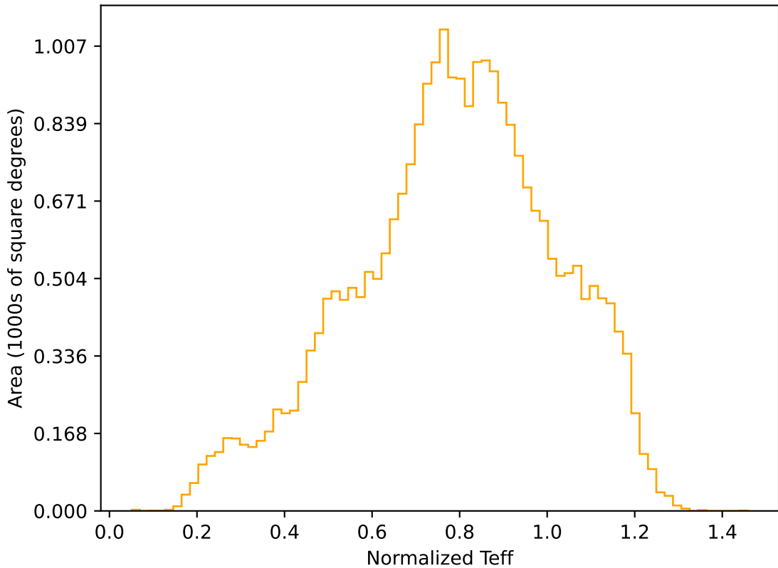
internal_u_expt45_nscale1.2v3.4_10yrs All sky r band: Normalized Teff
