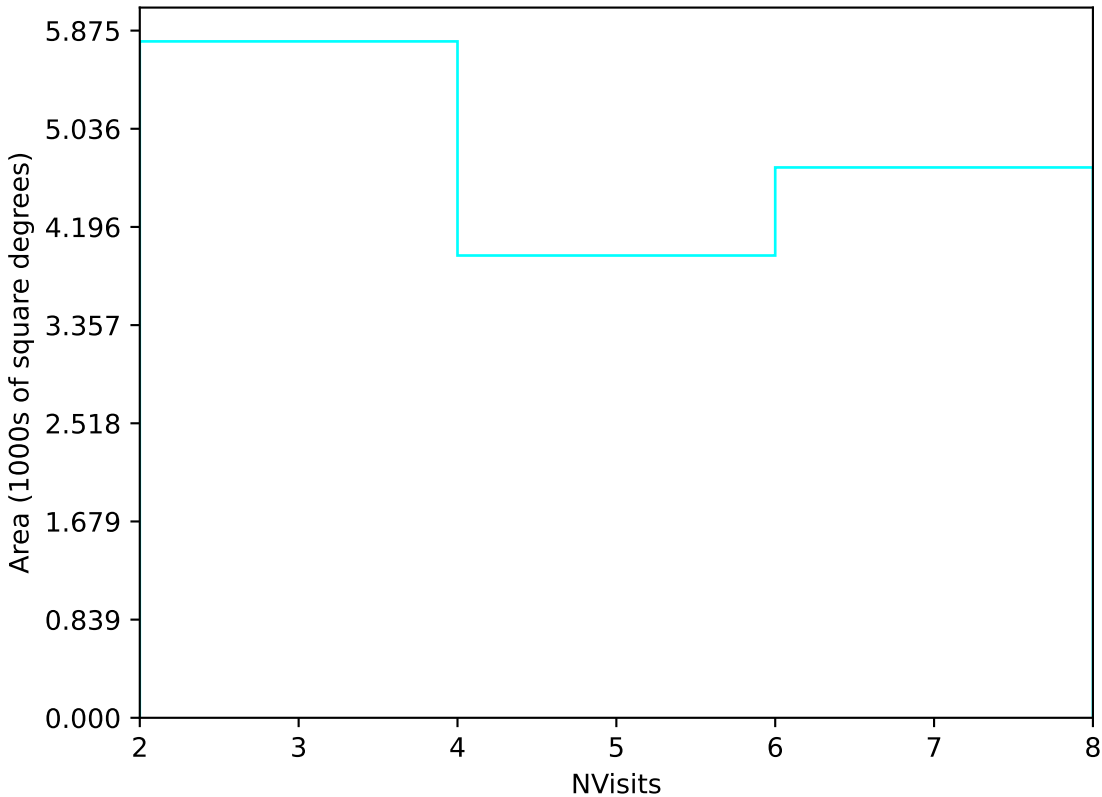
internal_u_expt45_nscale1.2v3.4_10yrs Yr 3-4 u band: NVisits
