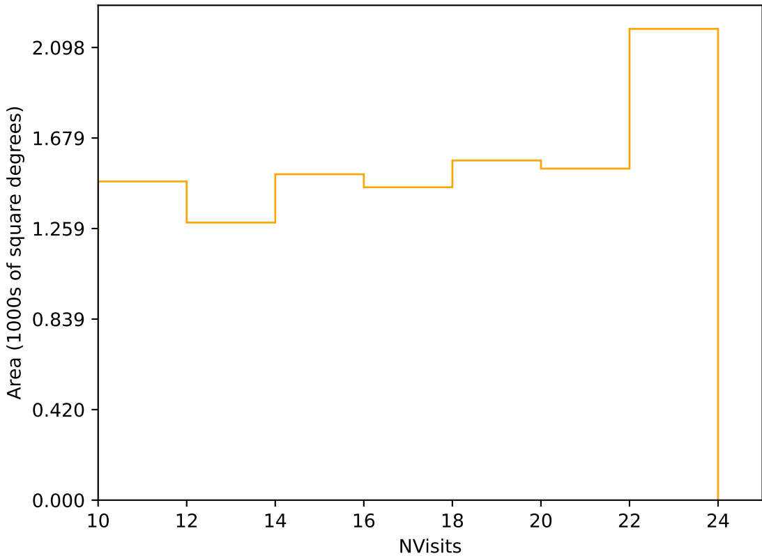
internal_u_expt45_nscale1.2v3.4_10yrs Yr 3-4 r band: NVisits
