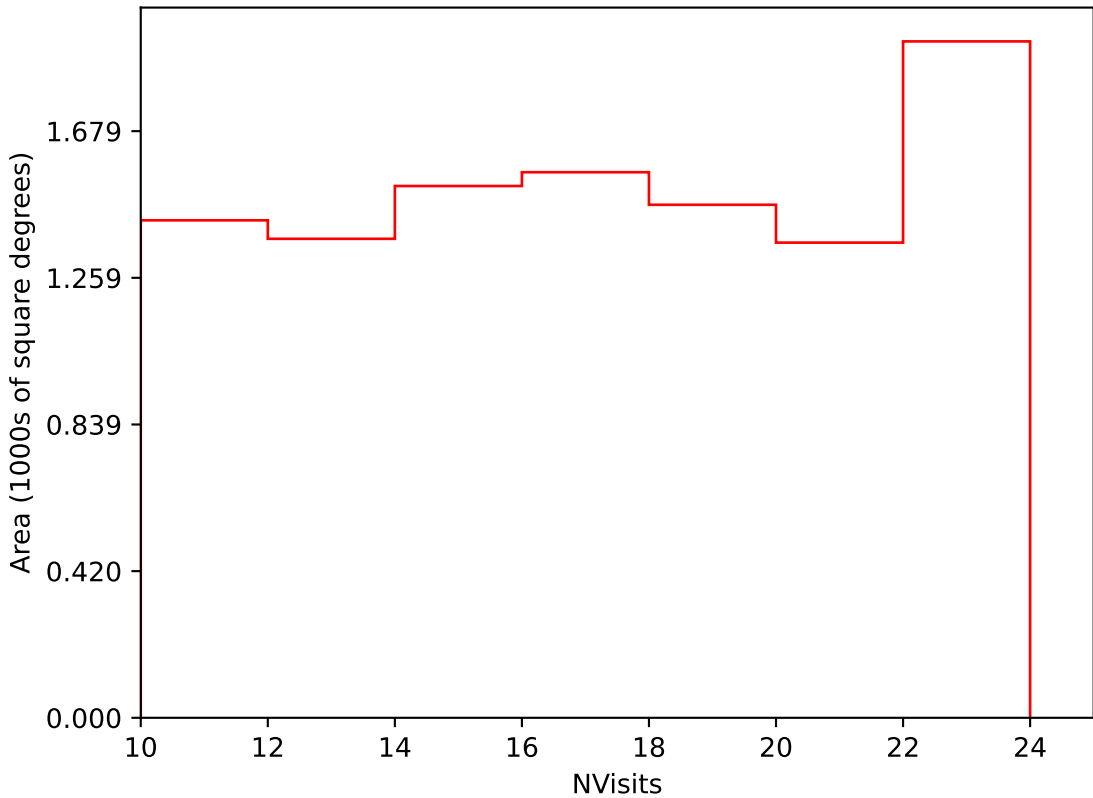
internal_u_expt45_nscale1.2v3.4_10yrs Yr 3-4 i band: NVisits
