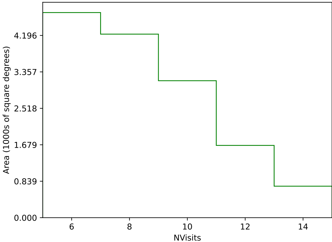
internal_u_expt45_nscale1.2v3.4_10yrs Yr 3-4 g band: NVisits
