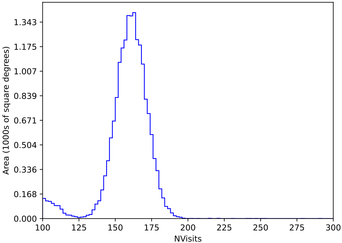
internal_u_expt45_nscale1.2v3.4_10yrs WFD y band: NVisits
