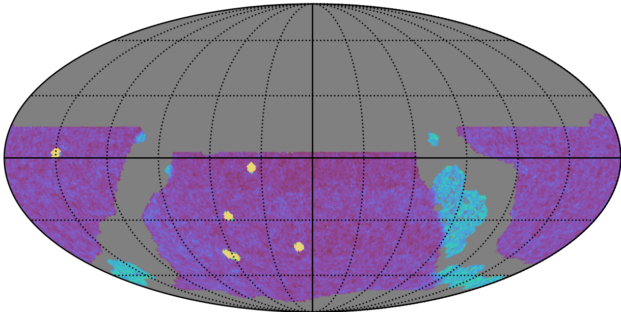
internal_u_expt45_nscale1.2v3.4_10yrs WFD g band: NVisits
