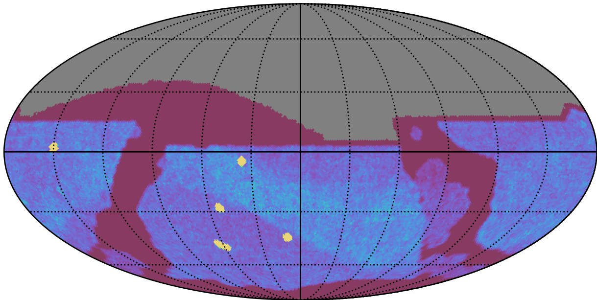
internal_u_expt45_nscale1.2v3.4_10yrs All sky z band: NVisits
