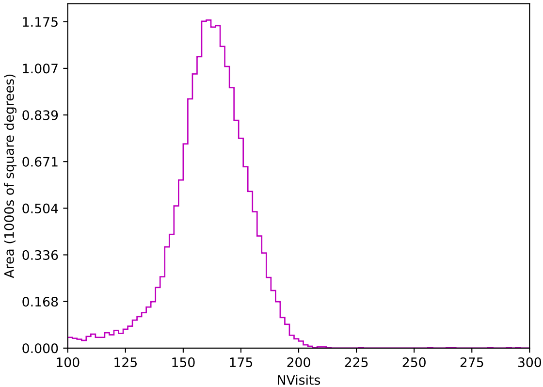
internal_u_expt45_nscale1.2v3.4_10yrs All sky z band: NVisits
