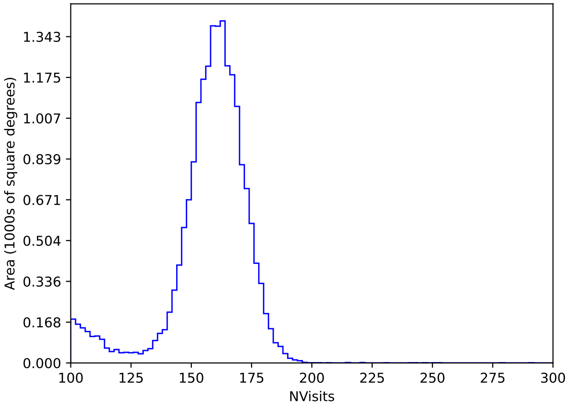
internal_u_expt45_nscale1.2v3.4_10yrs All sky y band: NVisits
