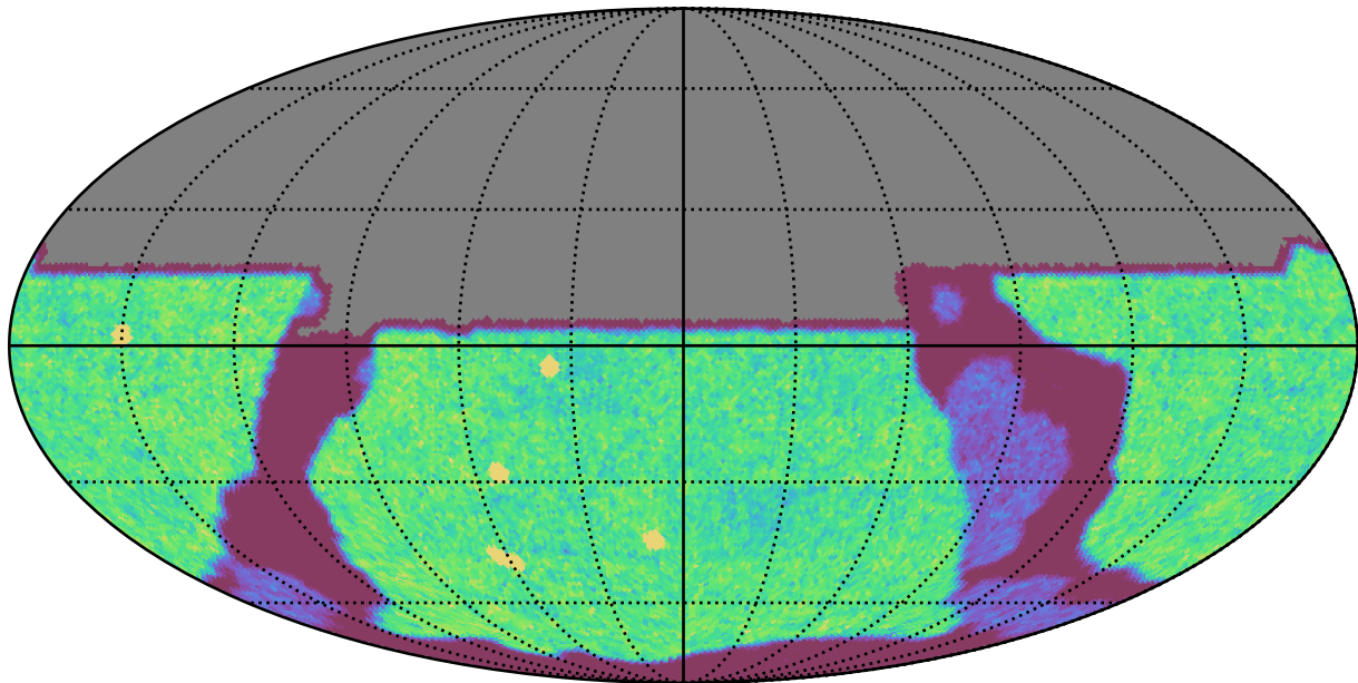
internal_u_expt45_nscale1.2v3.4_10yrs All sky u band: NVisits
