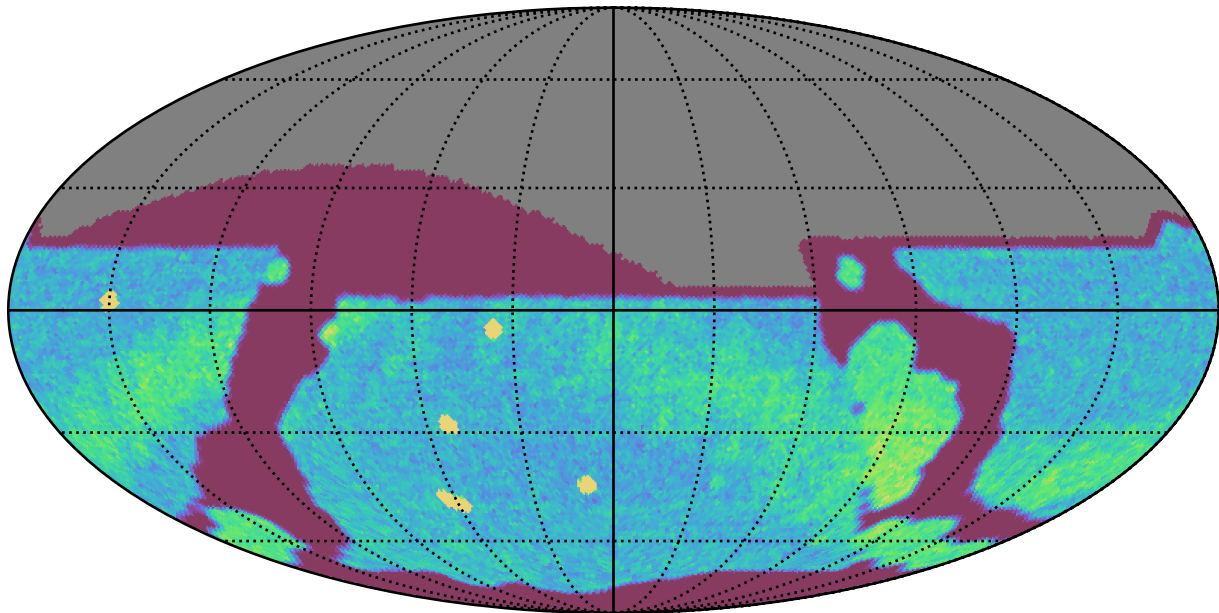
internal_u_expt45_nscale1.2v3.4_10yrs All sky r band: NVisits
