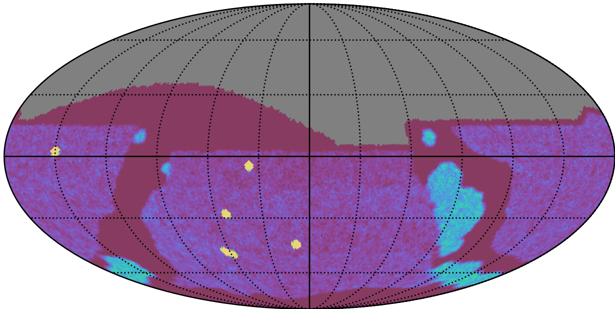
internal_u_expt45_nscale1.2v3.4_10yrs All sky g band: NVisits
