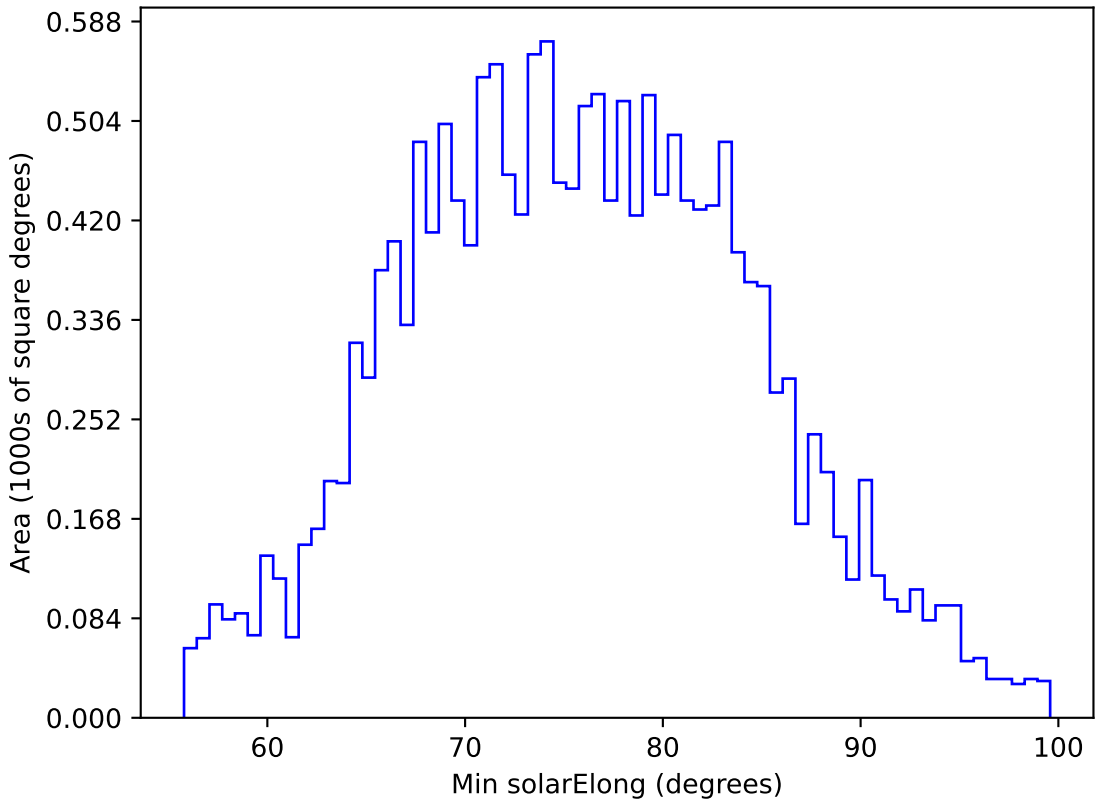
internal_u_expt45_nscale1.2v3.4_10yrs WFD g band: Min solarElong
