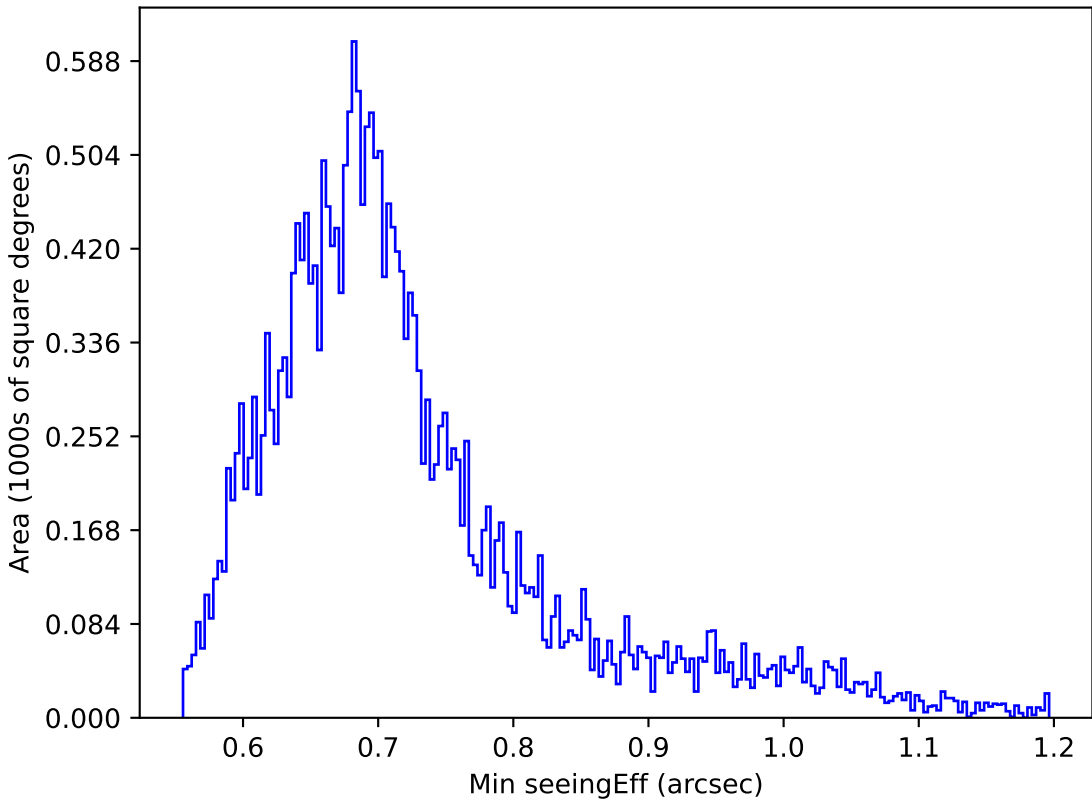
internal_u_expt45_nscale1.2v3.4_10yrs Yr 1 z band: Min seeingEff
