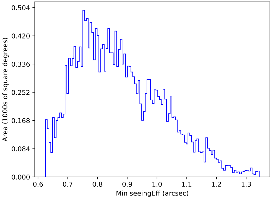
internal_u_expt45_nscale1.2v3.4_10yrs Yr 1 u band: Min seeingEff
