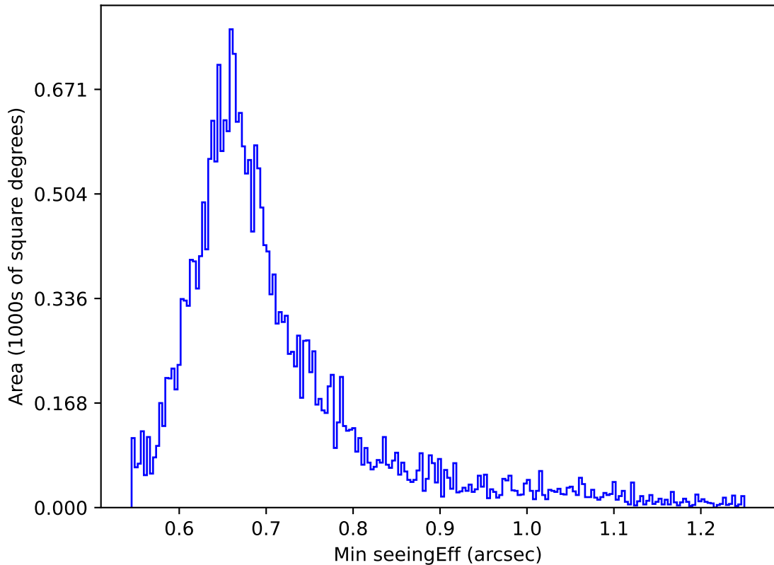
internal_u_expt45_nscale1.2v3.4_10yrs Yr 1 i band: Min seeingEff
