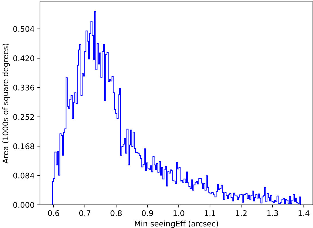
internal_u_expt45_nscale1.2v3.4_10yrs Yr 1 g band: Min seeingEff
