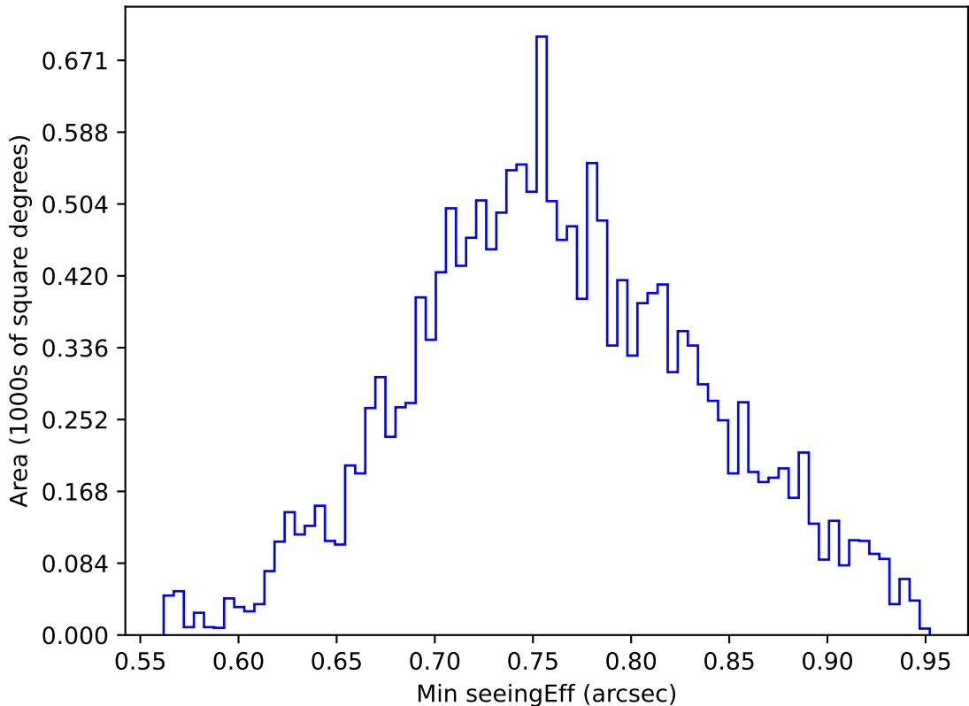
internal_u_expt45_nscale1.2v3.4_10yrs WFD u band: Min seeingEff
