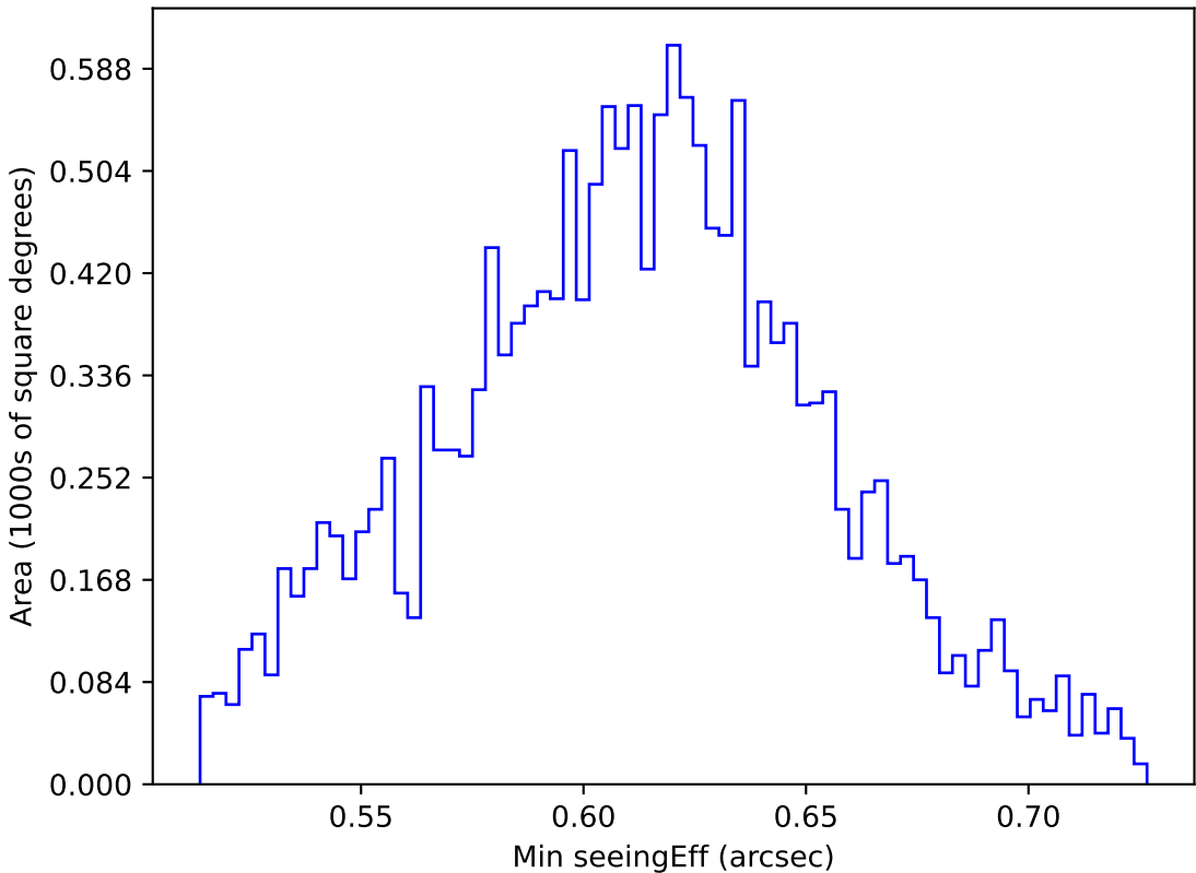
internal_u_expt45_nscale1.2v3.4_10yrs WFD r band: Min seeingEff
