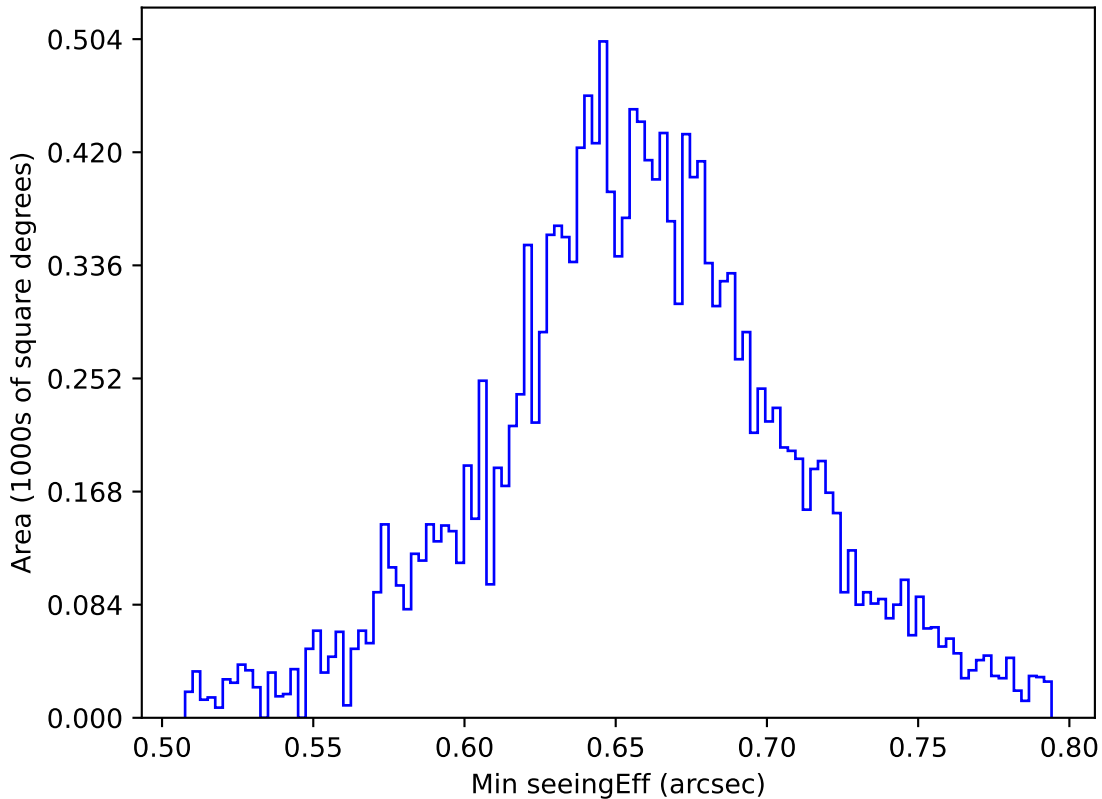
internal_u_expt45_nscale1.2v3.4_10yrs WFD g band: Min seeingEff
